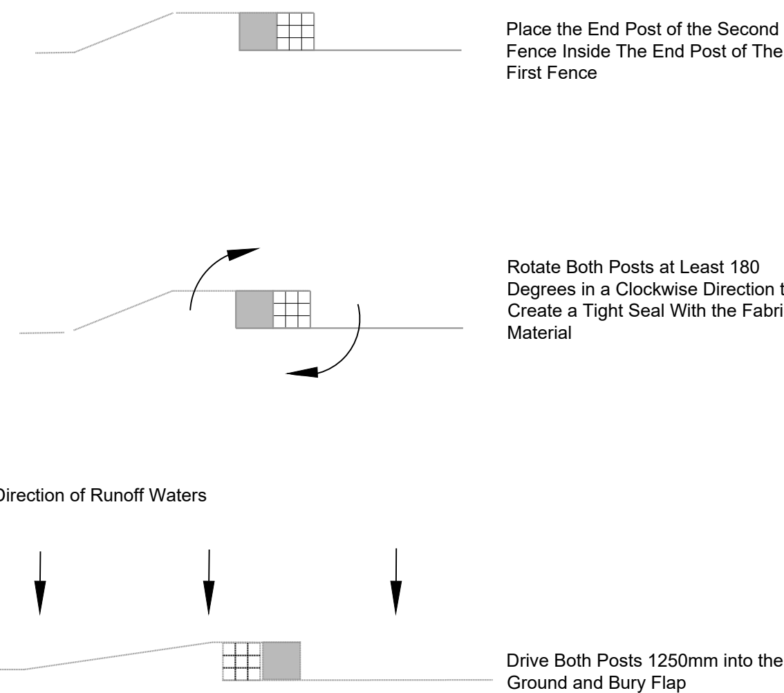
SILT FENCE DETAILS Scale 1:20
